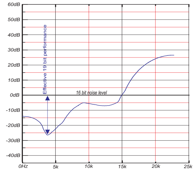
Noise shaper performance graphs at 16 bit output
